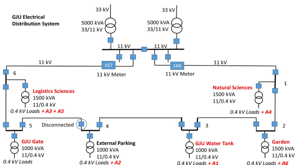
Figure 15: GJU Electrical one line diagram.
