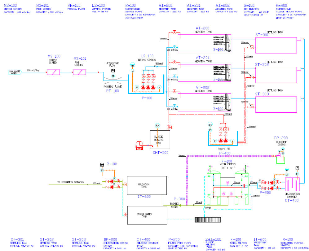
Figure 24: Wastewater treatment plant schematic.
